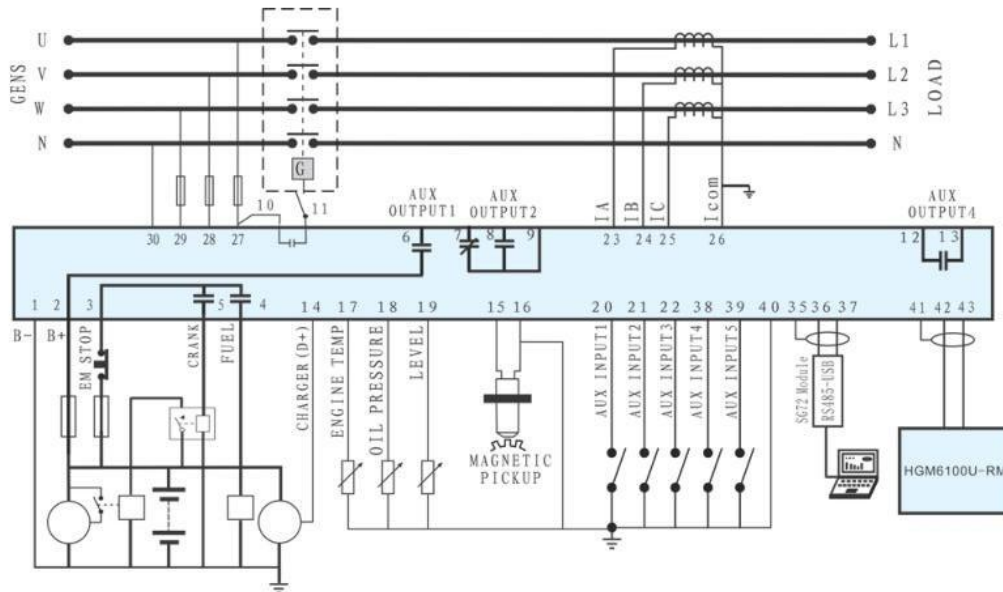
HGM6110U2C Typical Application Diagram
