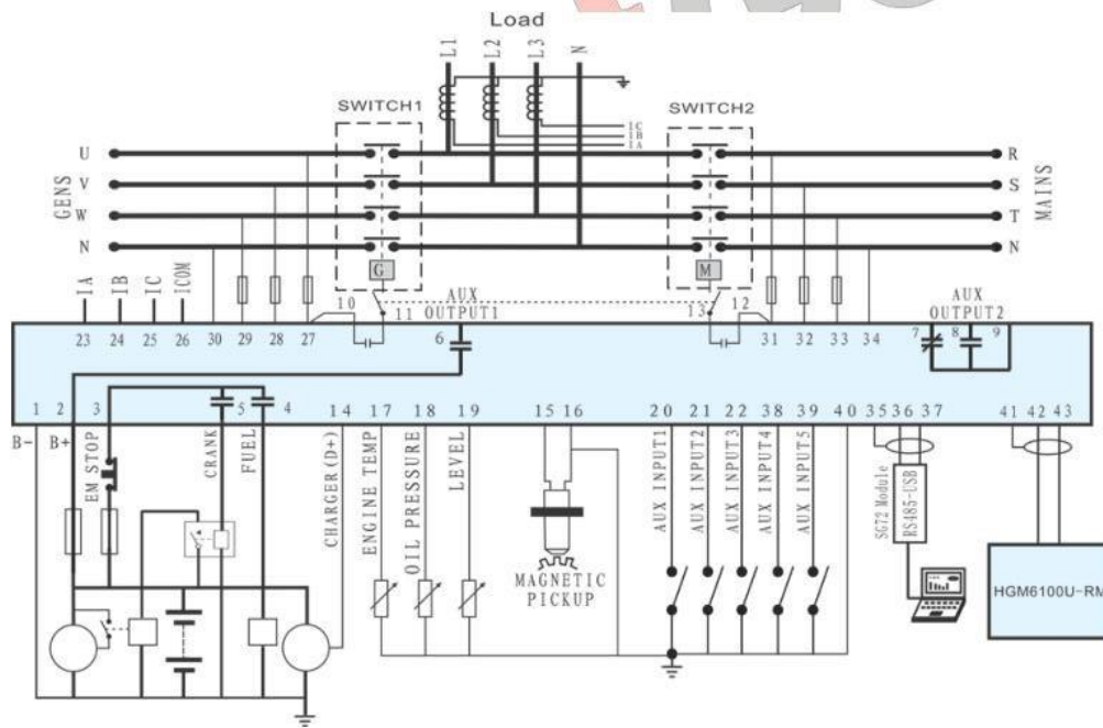
HGM6120U2C Typical Application Diagram
